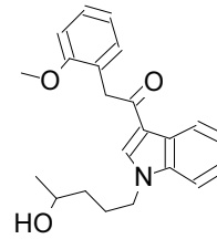
45 JWH-250 N-(...
