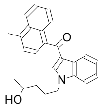
34 JWH-122 N-(...
