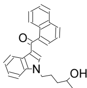
22 JWH-018 N-(...
