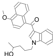
32 JWH-081 N-(...
