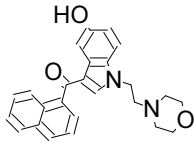
37 JWH-200 5-h...
