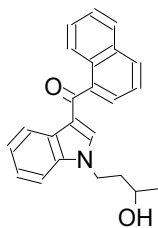
29 JWH-073 N-(...
