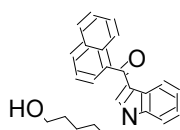
26 JWH-019 N-(...
