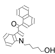
23 JWH-018 N-(...
