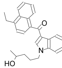
42 JWH-210 N-(...
