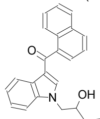
28 JWH-073 N-(...
