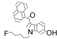
15 AM2201 6-hy...
