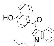
31 JWH-081 4-h...
