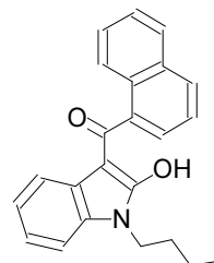
27 JWH-073 2-h...
