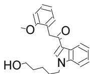
46 JWH-250 N-(...
