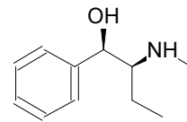
18 Buphedrone ...
