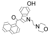
38 JWH-200 6-h...
