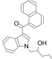
20 JWH-018 N-(...
