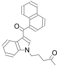
19 JWH 018 N-(...
