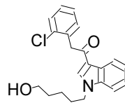
41 JWH-203 N-(...
