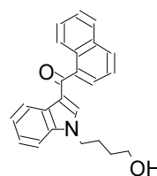
30 JWH-073 N-(...
