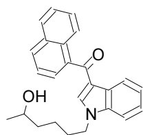
25 JWH-019 N-(...
