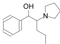
58 \alpha -Pyrrolidino...
