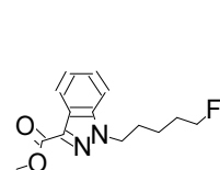
118 5F-AB-PINA...
