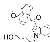
33 JWH-081 N-(...
