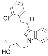
40 JWH-203 N-(...
