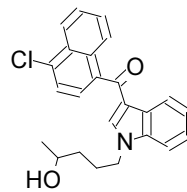
47 JWH-398 N-(...
