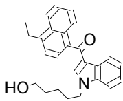
43 JWH-210 N-(...
