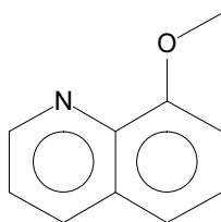
110 Quinoline, 8...
