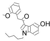
44 JWH-250 5-h...
