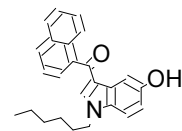
24 JWH-019 5-h...
