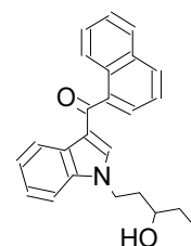
21 JWH-018 N-(...
