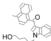
35 JWH-122 N-(...
