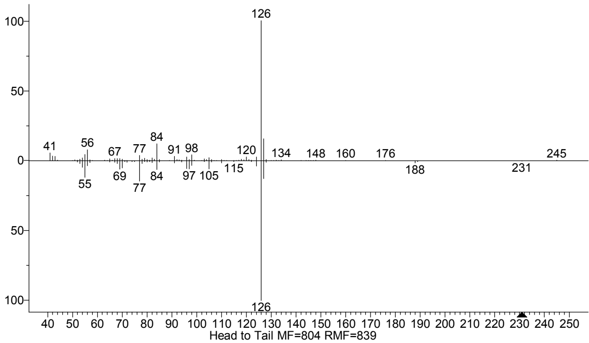
(Text File) Scan 1241 (10.645 min): reanim_79.D\data.ms (-1231)
